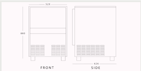
SIMAG SMI80 H 880mm W 529mm D 626mm
