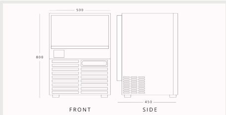
BLIZZARD BIM40 H 800mm W 500mm D 450mm
