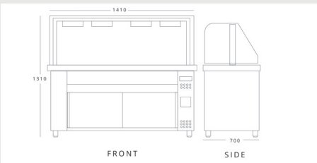
I NOKAK MFV714 (MIV714) H 1310mm W 1410mm D 700mm
