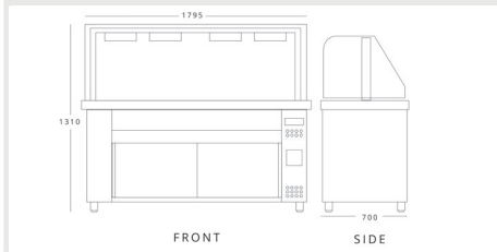
I NOKAK MFV718 (MIV718) H 1310mm W 1795mm D 700mm
