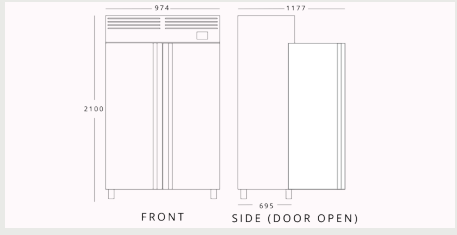
INFIRICO AGN602 H 2100mm W 974mm D 695mm
