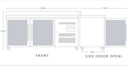
BLIZZARD HBC2CR H 950mm W 1360mm D 700mm
