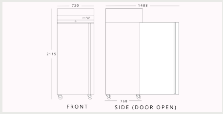
INOMAK CAP172SL(BK) H 2115mm W 720mm D 768mm
