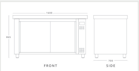
INOMAK HCP16 H 865mm W 1600mm D 700mm
