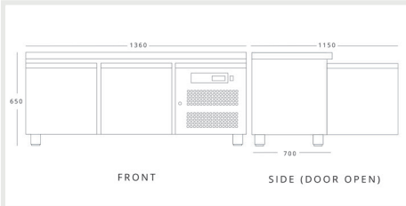
BLIZZARD SNC2 H 650mm W 1360mm D 700mm
