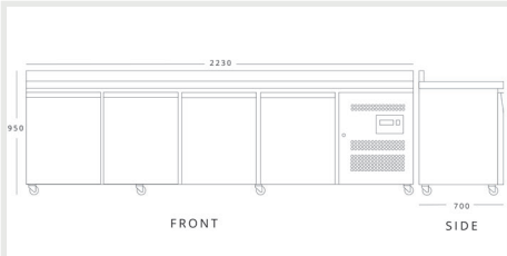
BLIZZARD LBC4 H 950mm W 2230mm D 700mm
