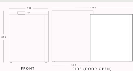
BLIZZARD UCR140 H 819mm W 598mm D 598mm
