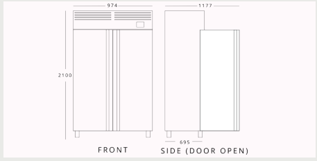
INFIRICO AGN602MIX H 2100mm W 974mm D 695mm
