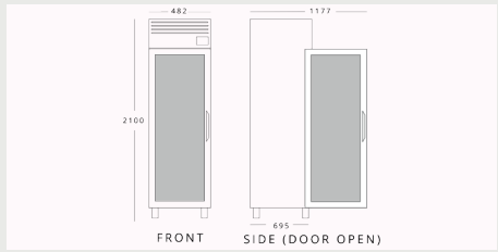
INFIRICO AGN300CR H 2100mm W 482mm D 695mm
