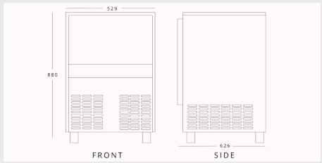
SIMAG SPH80 H 880mm W 529mm D 626mm
