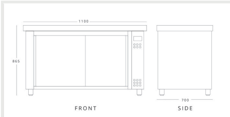
INOMAK HCP11 H 865mm W 1100mm D 700mm
