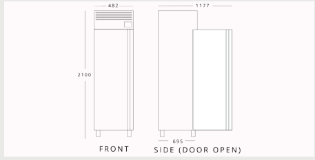
INFIRICO AGN301BT H 2100mm W 482mm D 695mm
