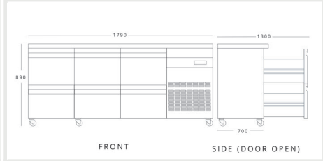
INOMAK PN222-HC H 890mm W 1790mm D 700mm
