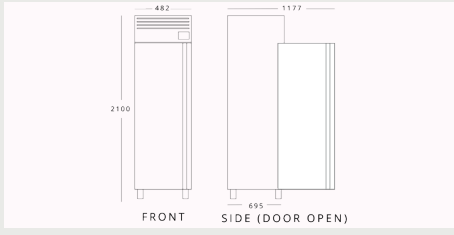
INFIRICO AGN301 H 2100mm W 482mm D 695mm
