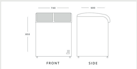
BLIZZARD BDF22 H 850mm W 740mm D 680mm
