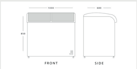
BLIZZARD BDF32 H 850mm W 1030mm D 680mm
