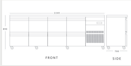
INOMAK PN2222-HC H 890mm W 2240mm D 700mm
