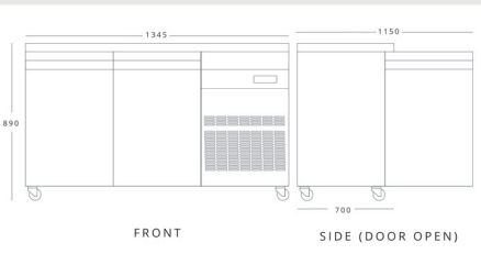
INOMAK PN99(BK)-HC H 890mm W 1345mm D 700mm
