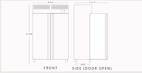
INFIRICO AGN602BT H 2100mm W 974mm D 695mm
