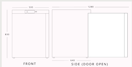
KOLDBOX KXR200 H 830mm W 595mm D 640mm
