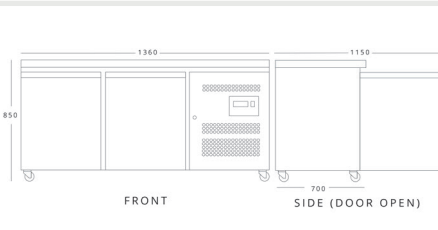
BLIZZARD HBC2NU H 850mm W 1360mm D 700mm
