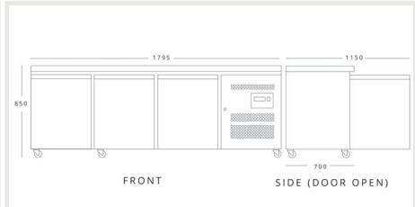
BLIZZARD HBC3NU H 850mm W 1795mm D 700mm
