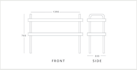
INOMAK RD314 H 765mm W 1390mm D 333mm
