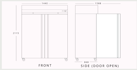
INOMAK CEP2144(BK) H 2115mm W 1440mm D 868mm
