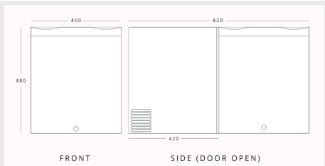
BLIZZARD BMB30 H 480mm W 400mm D 420mm
