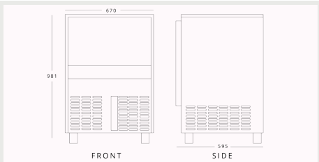
SIMAG SDH100 H 981mm W 670mm D 595mm
