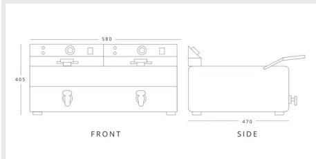
BLIZZARD BF8+8 H 405mm W 580mm D 470mm
