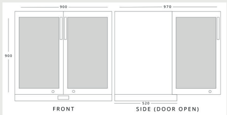
KOLDBOX KBC2 H 900mm W 900mm D 520mm
