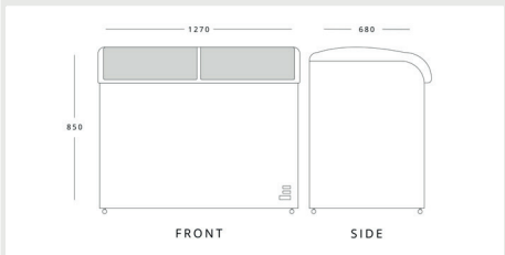
BLIZZARD BDF42 H 850mm W 1270mm D 680mm
