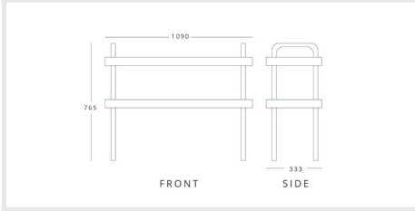
INOMAK RD311 H 765mm W 1090mm D 333mm
