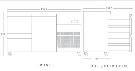
INOMAK PN29-HC H 890mm W 1345mm D 700mm
