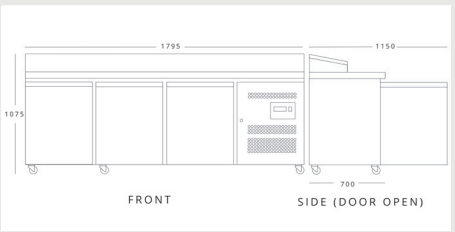
BLIZZARD HBC3EN H 1075mm W 1795mm D 700mm
