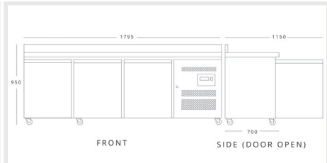
BLIZZARD LBC3 H 950mm W 1795mm D 700mm
