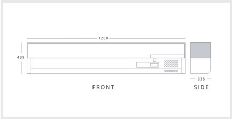
BLIZZARD TOP1200-14CR H 439mm W 1200mm D 395mm
