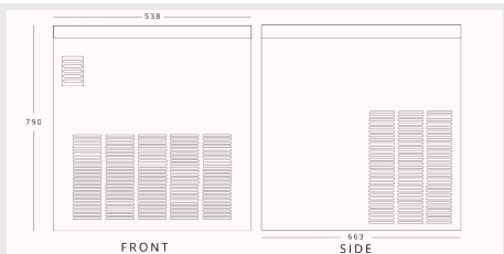
SIMAG SPN605 H 790mm W 538mm D 663mm
