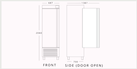
INFIRICO AN501TF H 2060mm W 687mm D 700mm
