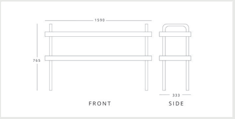
INOMAK RD316 H 765mm W 1590mm D 333mm
