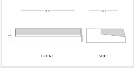
MAFIROL HERA FISH 1500 SB-VBS H 400mm W 1510mm D 1035mm
