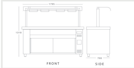
I NOKAK MVV718 (MJV718) H 1310mm W 1795mm D 700mm
