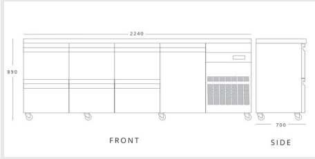
INOMAK PN2229-HC H 890mm W 2240mm D 700mm
