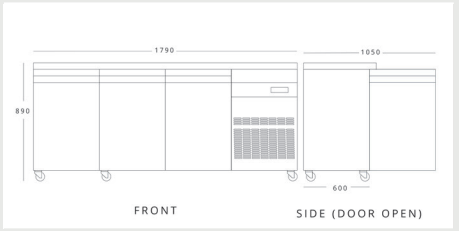
INOMAK SL999-HC H 890mm W 1790mm D 600mm
