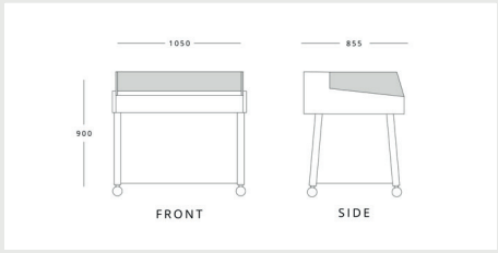
MAFIROL HERA FISH SS 1040 CB-VBS H 900mm W 1050mm D 855mm
