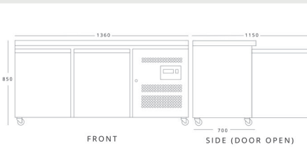
BLIZZARD LBC2NU H 850mm W 1360mm D 700mm
