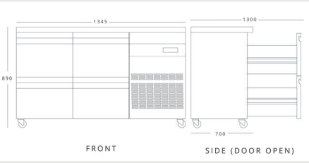
INOMAK PN22-HC H 890mm W 1345mm D 700mm
