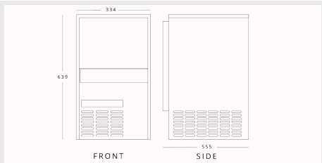
SIMAG SDH34 H 639mm W 334mm D 555mm
