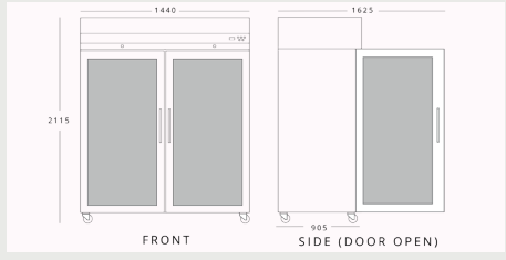
INOMAK CFP2144CR(BK) H 2115mm W 1440mm D 905mm
