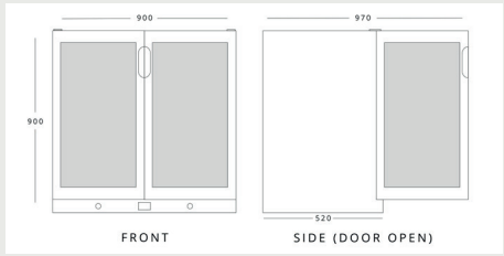
INFRICO ZX2(SS) H 900mm W 900mm D 520mm
