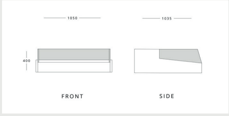
MAFIROL HERA FISH 1040 SB-VBS H 400mm W 1050mm D 1035mm
