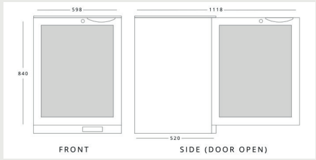
BLIZZARD LOWBAR1 H 840mm W 598mm D 520mm
