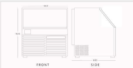
BLIZZARD BIM90 H 920mm W 660mm D 685mm
