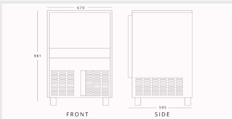
SIMAG SDH84 H 981mm W 670mm D 595mm
