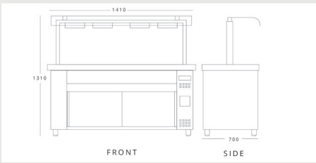
I NOKAK MVV714 (MJV714) H 1310mm W 1410mm D 700mm
