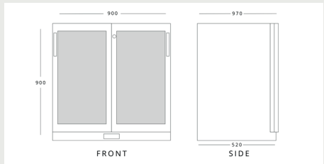
INFRICO ZX2-SL H 900mm W 900mm D 520mm
