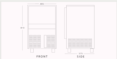
SIMAG SDH50 H 810mm W 485mm D 575mm
