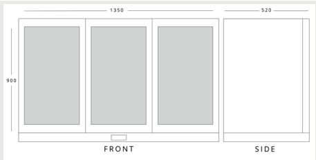
KOLDBOX KBC3SL H 900mm W 1350mm D 520mm
