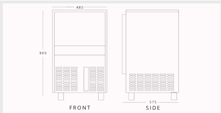
SIMAG SDH64 H 905mm W 485mm D 575mm
