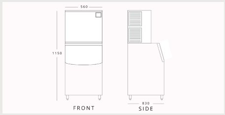
BLIZZARD BIM160 H 1150mm W 560mm D 830mm
