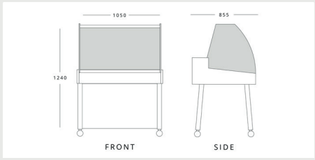
MAFIROL HERA FISH SS 1040 CB-VCR H 1240mm W 1050mm D 855mm
