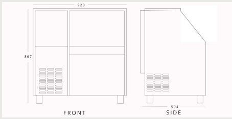
SIMAG SPH200 H 867mm W 920mm D 594mm
