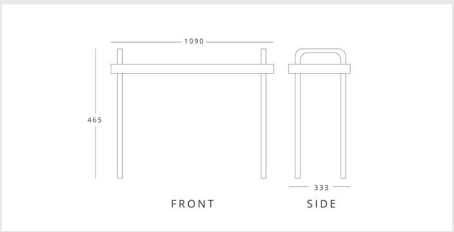
INOMAK RE311 H 465mm W 1090mm D 333mm
