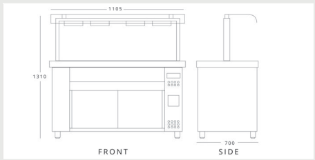
I NOKAK MVV711 (MJV711) H 1310mm W 1105mm D 700mm
