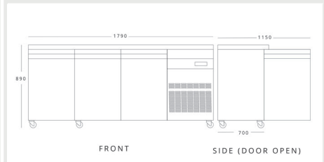
INOMAK PN999(BK)-HC H 890mm W 1790mm D 700mm
