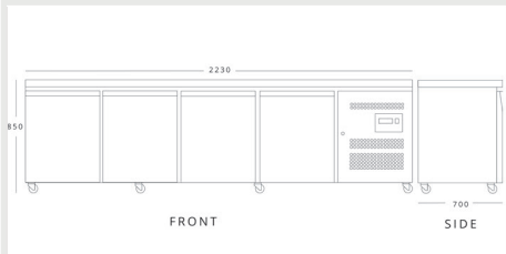
BLIZZARD HBC4NU H 850mm W 2230mm D 700mm
