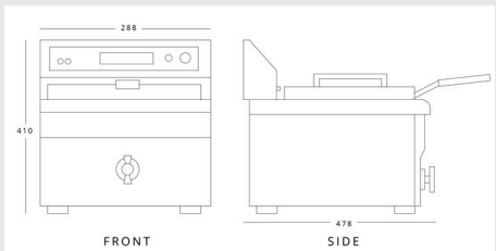
BLIZZARD BIF H 410mm W 288mm D 478mm
