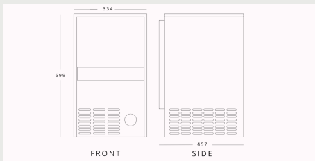
SIMAG SDH24 H 599mm W 334mm D 457mm
