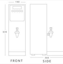
BLIZZARD AF10 H 630mm W 190mm D 360mm
