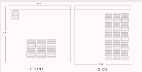
SIMAG SPN255 H 531mm W 564mm D 536mm
