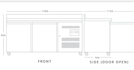
BLIZZARD LBC2 H 950mm W 1360mm D 700mm
