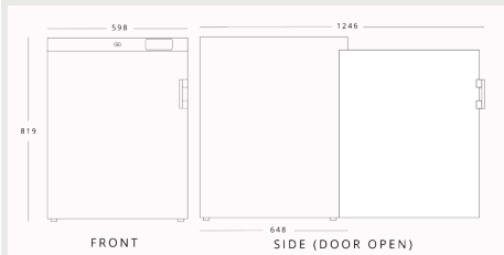
BLIZZARD UCR140WH H 819mm W 598mm D 648mm
