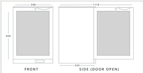
BLIZZARD BAR1(SS) H 900mm W 598mm D 520mm
