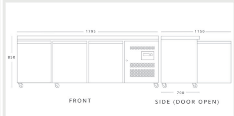
BLIZZARD LBC3NU H 850mm W 1795mm D 700mm
