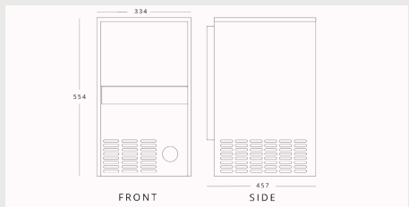
SIMAG SDH18 H 554mm W 334mm D 457mm
