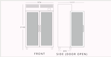
INFIRICO AGN600CR H 2100mm W 974mm D 695mm
