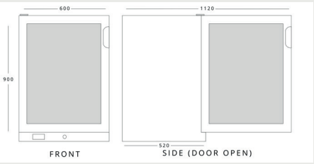
INFRICO ZX1(SS) H 900mm W 600mm D 520mm
