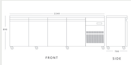
INOMAK PN9999(BK)-HC H 890mm W 2240mm D 700mm
