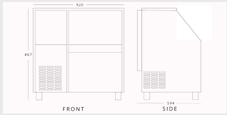
SIMAG SPH120 H 867mm W 920mm D 594mm
