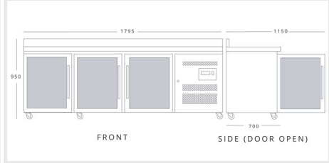
BLIZZARD HBC3CR H 950mm W 1795mm D 700mm
