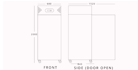
KOLDBOX KXF600 H 2000mm W 680mm D 840mm
