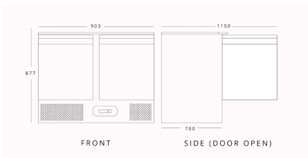
KOLDBOX KXCC2-PREP H 877mm W 903mm D 700mm
