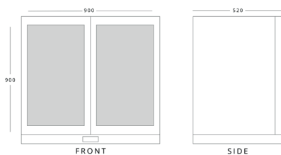
KOLDBOX KBC2SL H 900mm W 900mm D 520mm
