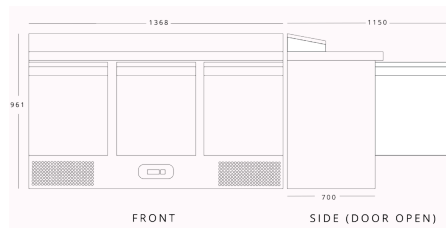
KOLDBOX KXCC3-SAL H 961mm W 1368mm D 700mm
