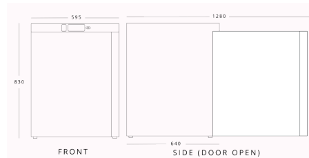
KOLDBOX KXF200 H 830mm W 595mm D 640mm
