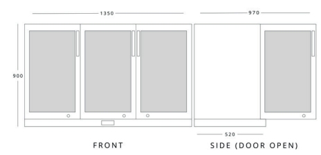
KOLDBOX KBC3 H 900mm W 1350mm D 520mm
