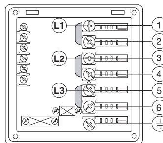
Figure 13 220-240V 3
