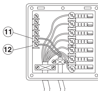
Figure 15 Energy control
