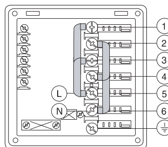
Figure 14 220-240V 1N
