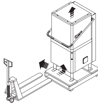
Figure 6 Machine positioning
