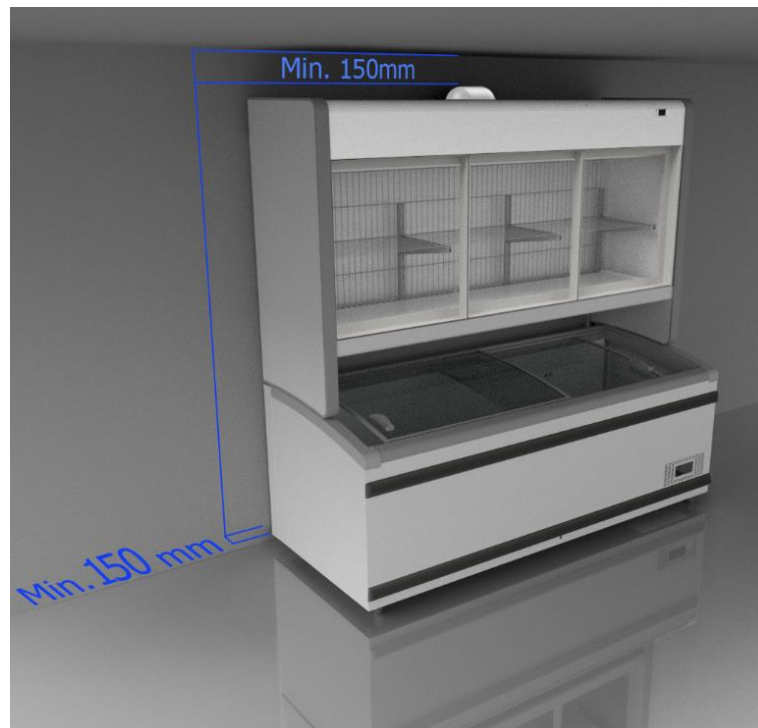
Fig.2 – Minimum installation distances
